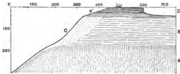
FIG. 173.—Section of the outer edge of one of the Maldivian Atolls. A , foundation of primitive rock cut down by the currents; B , upgrowth of the rim by the deep-sea-, intermediate depth- and ( B' ) reef-organisms; C , extension outwards by means of the talus slope; D , lagoon. Scale in fathoms. (After Stanley Gardiner.)
